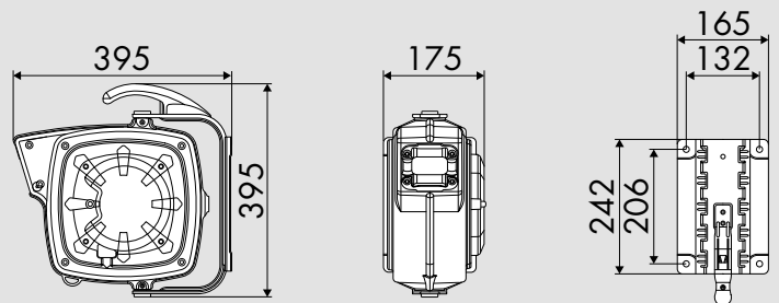
Overall dimensions with bayonet bracket (mm)
